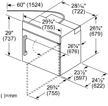
30" Single Oven Wall-Mounted Installation
