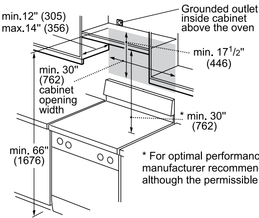
800 / 500 Series Cutout and Clearances
