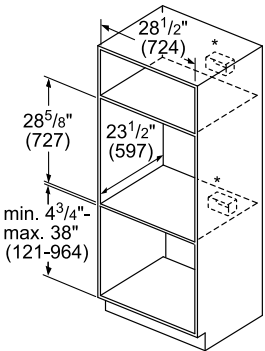
30" Speed Oven Over Warming Drawer
