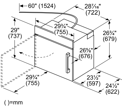
30" Single Oven Under-Counter Installation
