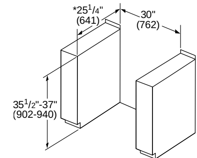
Gas Cutout Dimensions
