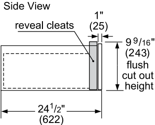
Flush Installation
