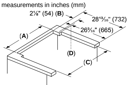
Downdraft Hood with Gas Rangetop Cutout
