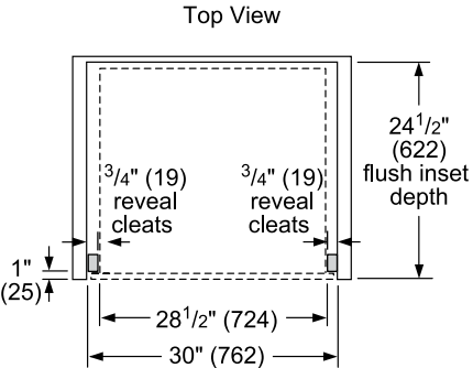
30" Flush Installation
