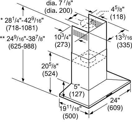
24" HCP34E52UC Pyramid Canopy Chimney Hood
