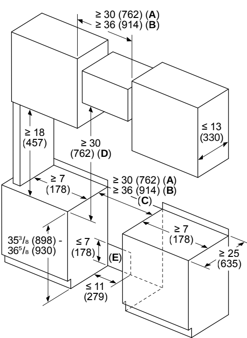
Industrial Style Range Installation
