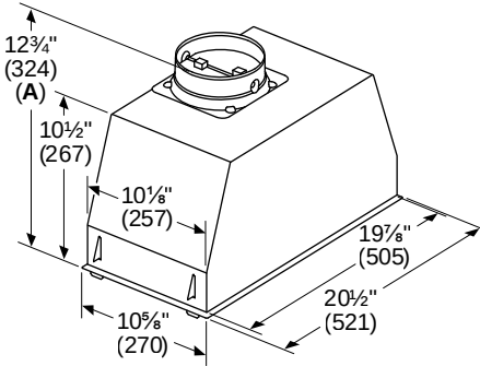
24" HUI34253UC Custom Insert Hood Dimensions
