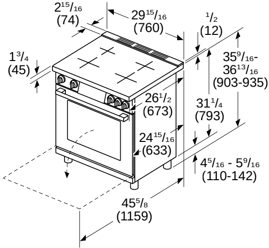
Industrial Style Range Installation
