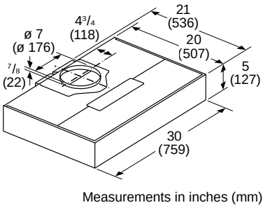
300 Series 30" DUH30253UC Under-Cabinet Hoods
