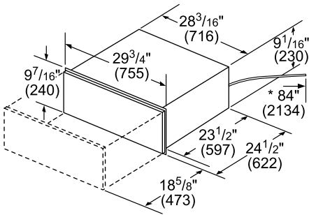
30" Warming Drawer Dimensions
