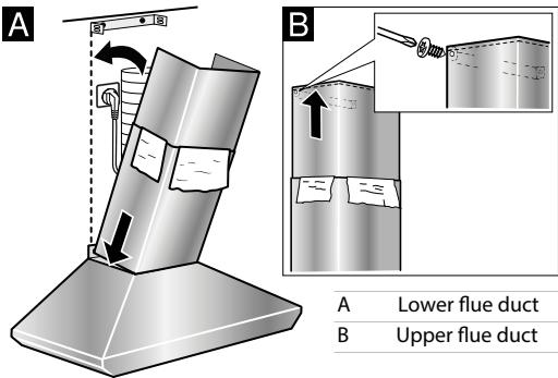
30" and 24" Pyramid Canopy Chimney Hoods
