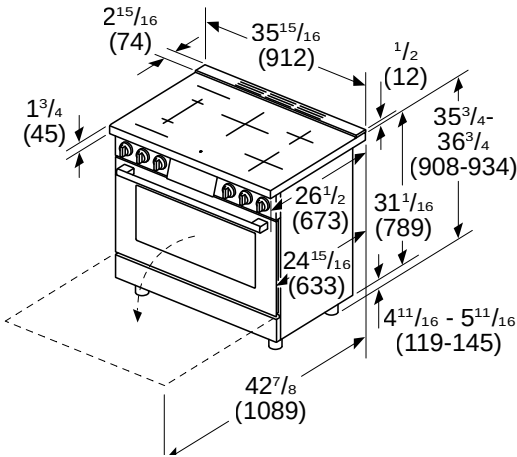
Industrial Style Range Dimensions
