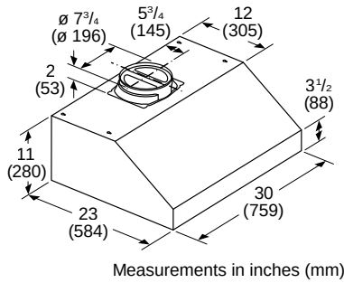
800 Series 30" DUH80553UC Under-Cabinet Hood
