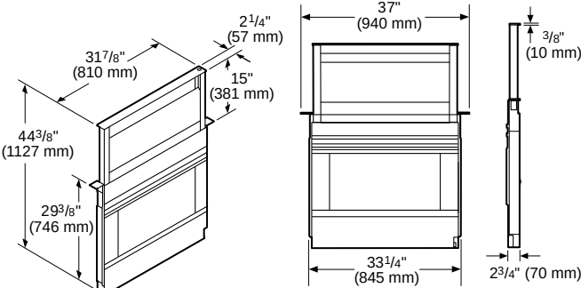
36" HDD86052UC Downdraft Hood
