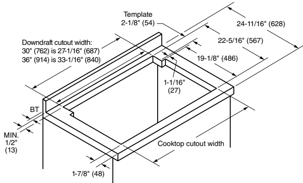
Downdraft Hood with Gas Rangetop Cutout
