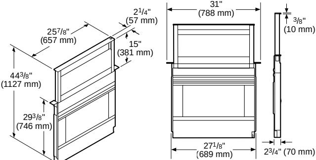
30" HDD80052UC Downdraft Hood
