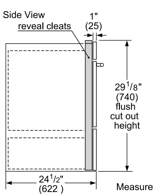
Speed Oven Over Warming Drawer
