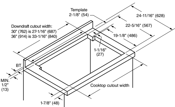
Downdraft Hood with Electric or Induction Cooktop Cutout
