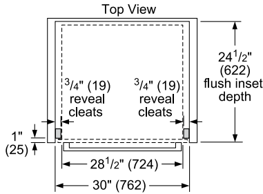
Flush Installation
