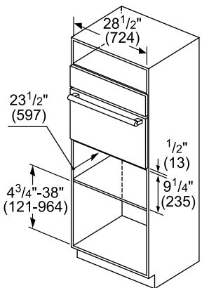
30" Warming Drawer Wall-Mounted
