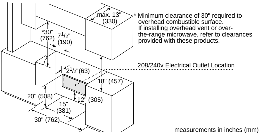
Induction & Electric Range Installation
