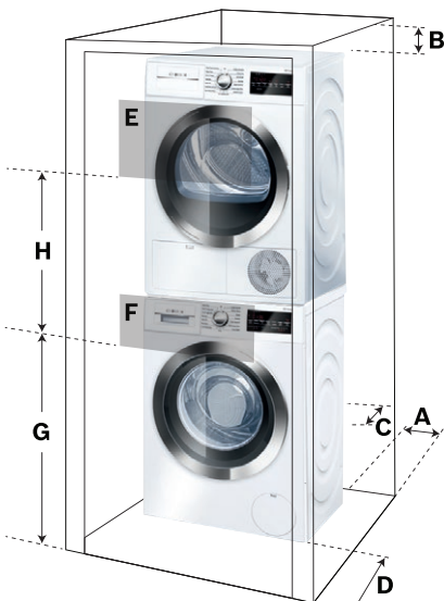
Closet: Stacked
