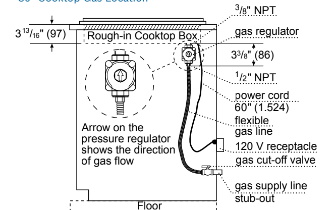
30" Cooktop Gas Location
