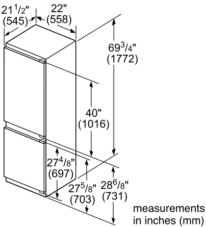
B09IB91NSP Installation
