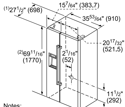
B20CS30SNS Dimensions
