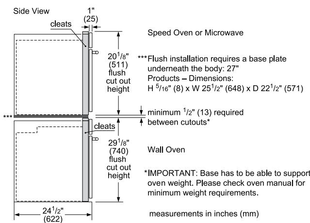
Flush Installation Speed Oven or Microwave over 27" Single Oven
