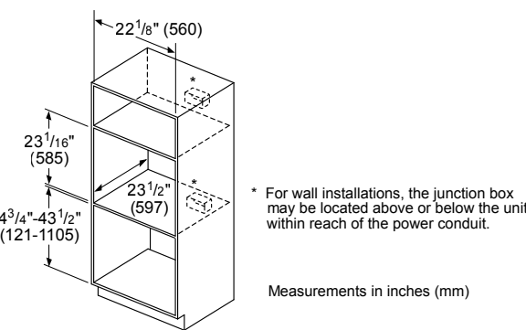
HBE5452UC Single Oven Wall-Mounted Installation
