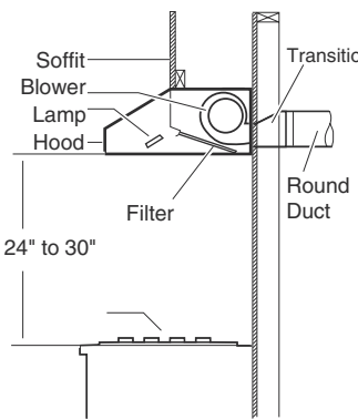
Horizontal discharge
