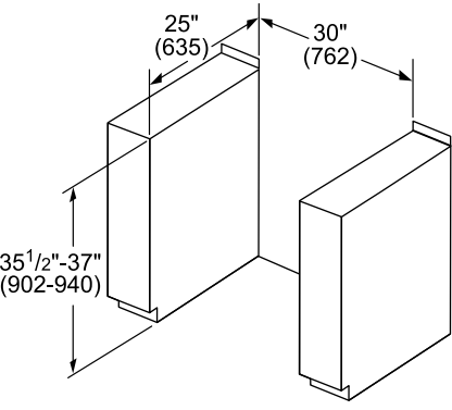
Electric Range Cutout Dimensions
