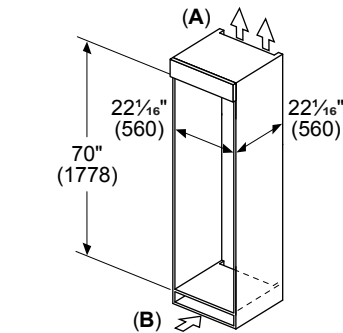
B09IB91NSP Installation
