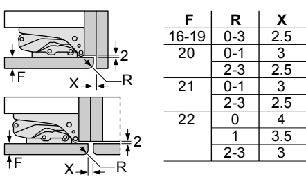
Recommended Gap Dimensions for Flat Hinges
